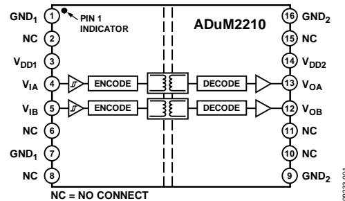
Figure 1. ADuM2210
