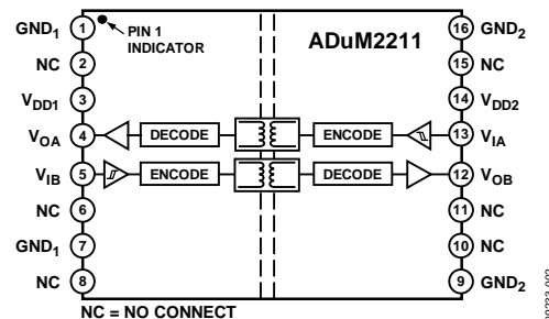
Figure 2. ADuM2211
